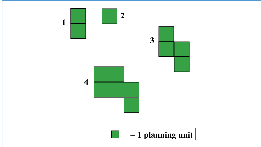
Figure 4-2. Hypothetical network of priority areas for conservation. For simplicity, only the planning units that were selected for the network are shown.
