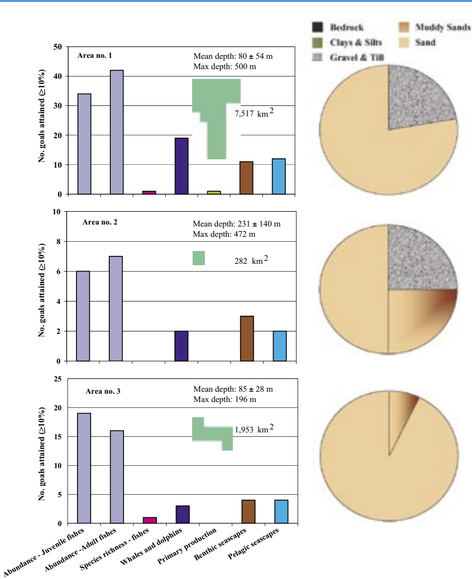
Figure E-1, below: Summaries of all 30 priority areas for conservation in terms of their contributions to the goals for the different classes of conservation features (histograms) and their seafloor characteristics (pie charts). Histogram bars show the total number of conservation features to which each priority area for conservation contributed \geq 10\% of the goal, within each of the classes of conservation features. Note that total number of conservation features was highest for those priority areas for conservation that spanned more than one biogeographic area because goals were set for each. There were many more conservation features for fishes and seascapes than for the other classes. There was just one conservation feature for primary production per biogeographic area, as was the case for fish species richness. Note, there were no cetacean conservation features for the Scotian Shelf biogeographic area due to incomplete data (*).
