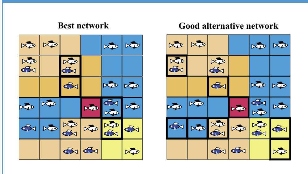
Figure 4-3. Two networks from a simple hypothetical MARXAN analysis, each of which meets the goals for habitat and biological conservation features: networks are comprised of the outlined planning units.
