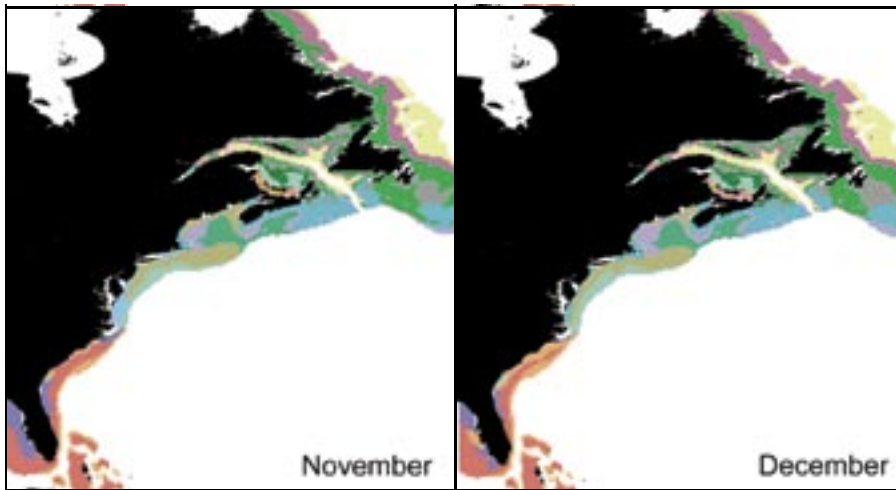
Figure D-2. Benthic temperature and salinity clusters (30 clusters), January to December. (Continued)
